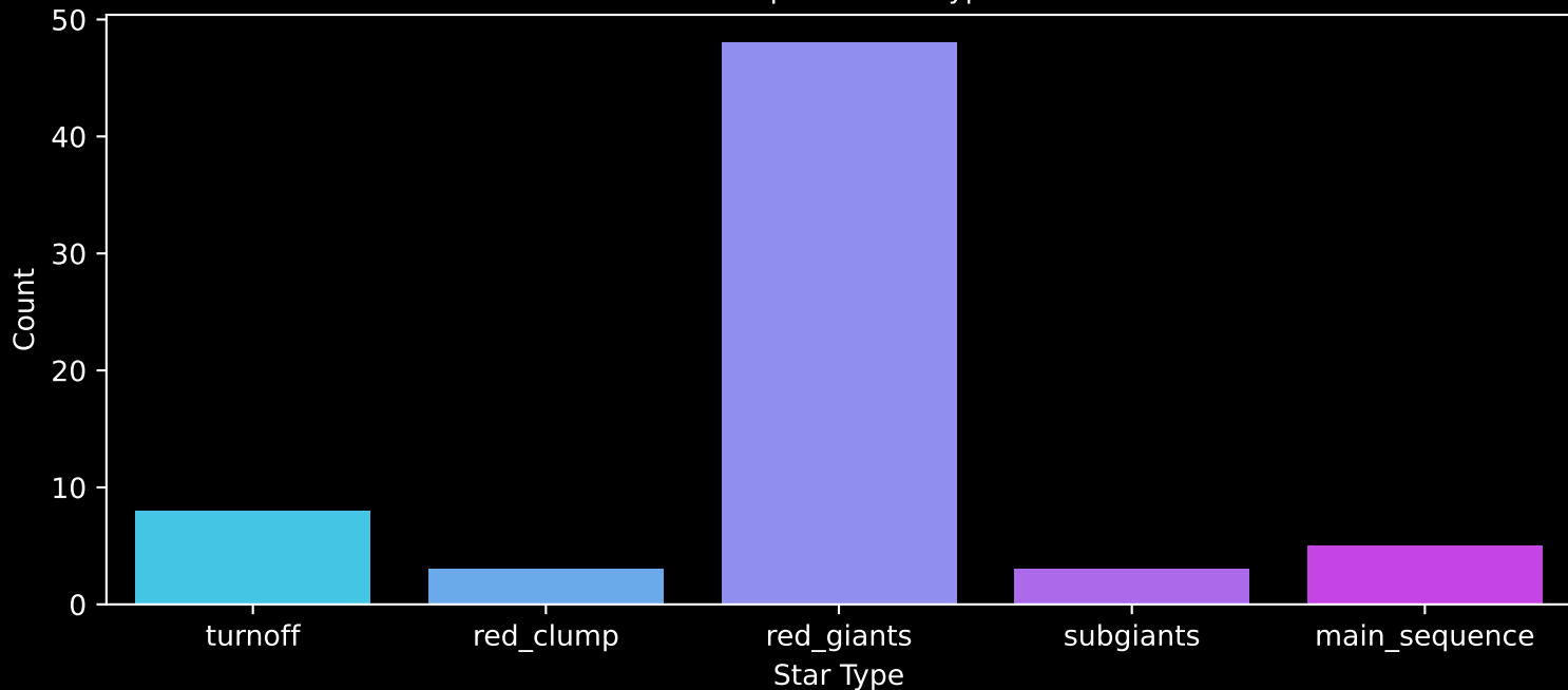
APOGEE DR17 Field: [LMC9] Count plot of Star Type
