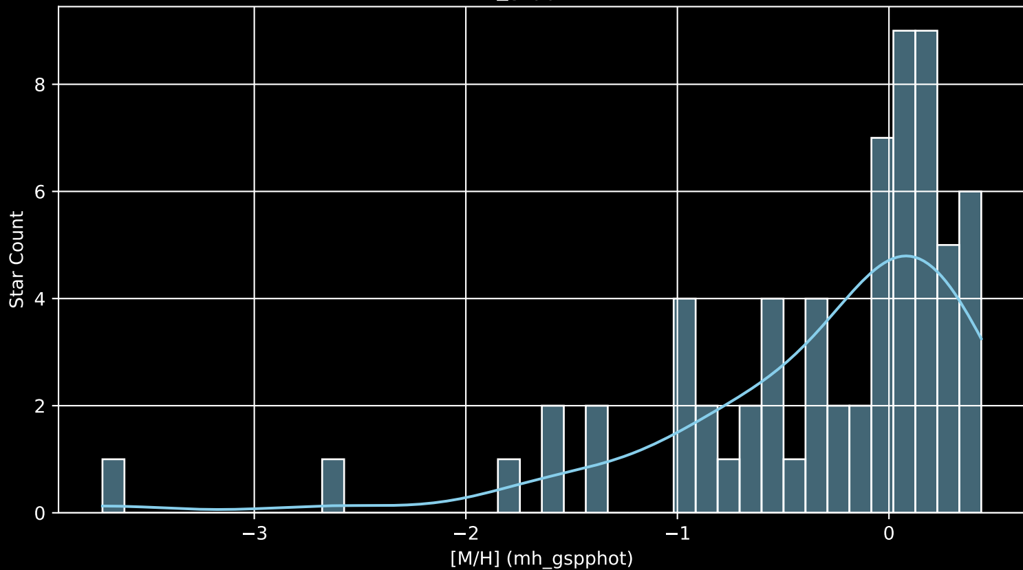
APOGEE DR17 Field: [LMC9 [M/H] (mh_gspphot) (n= 65)
