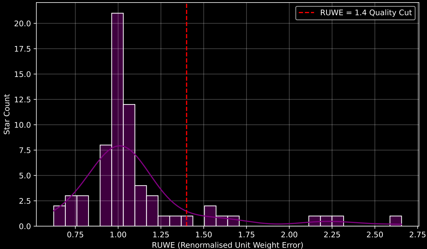
GAPOGEE DR17 Field [LMC9] RUWE Distribution (n= 67)
