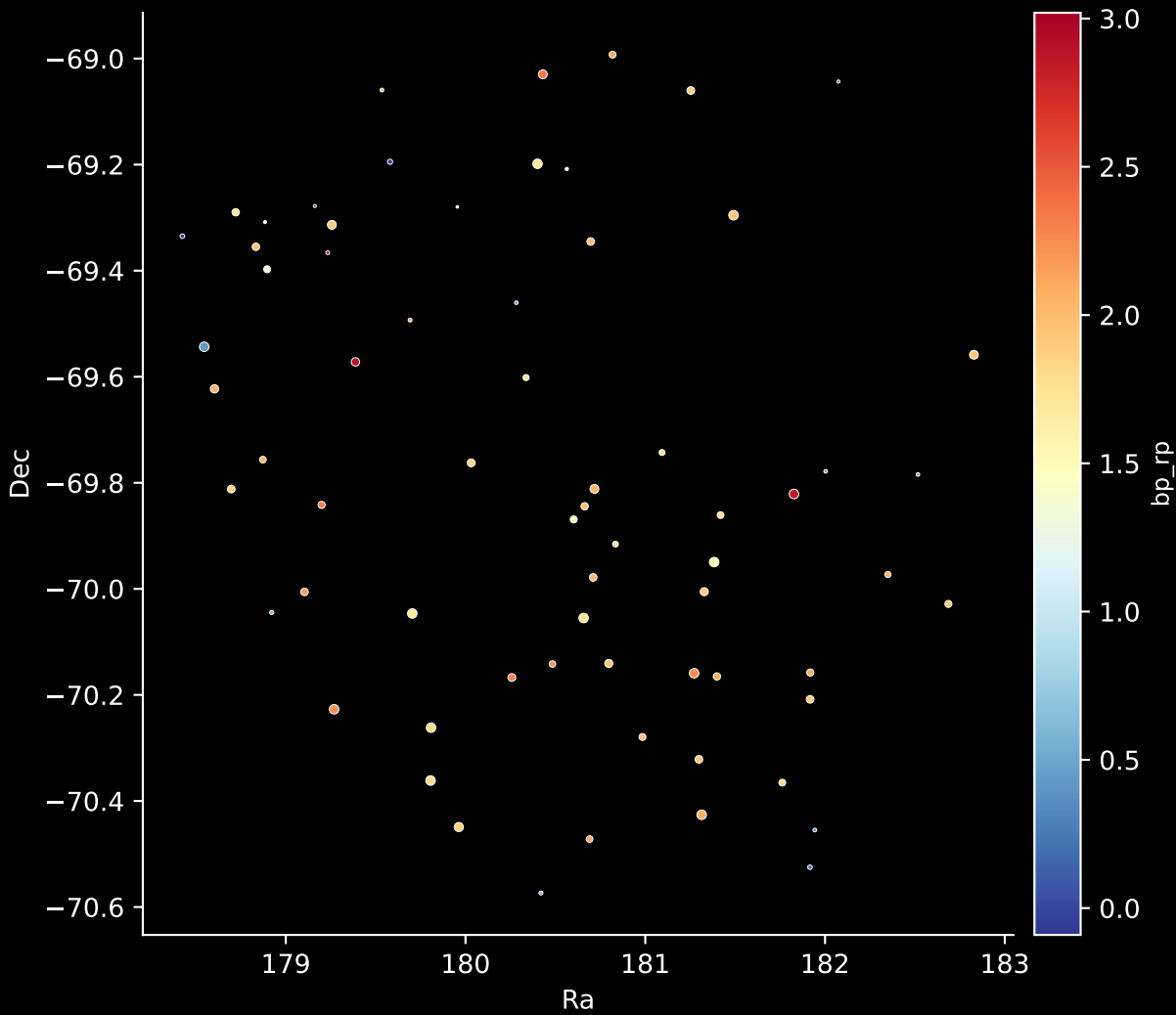
APOGEE DR17 Field: [LMC9] Stars: 67
