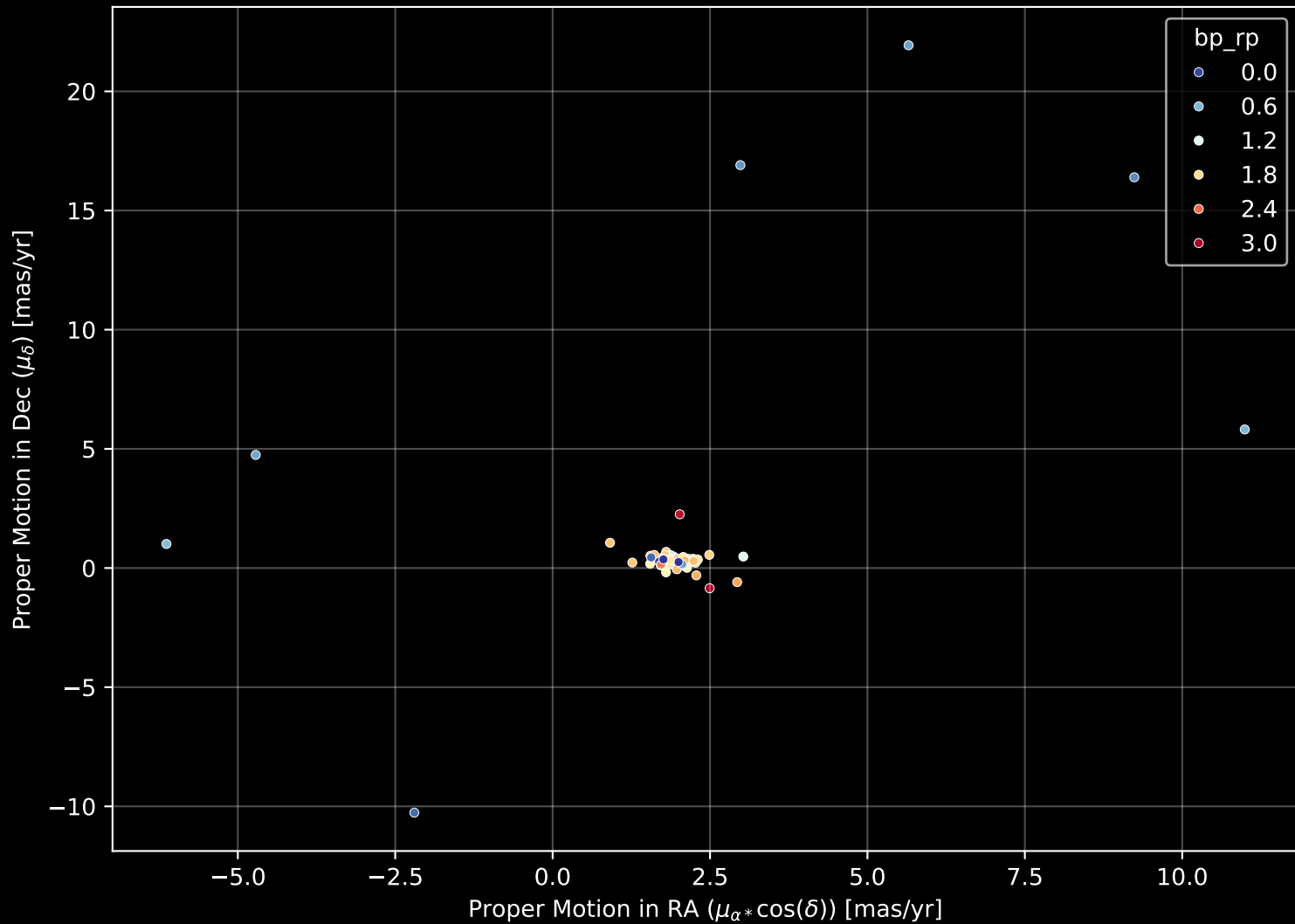
APOGEE DR17 Field: [LMC9] Proper Motion Diagram (n= 67)
