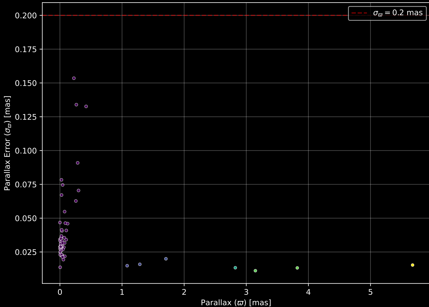
APOGEE DR17 Field: [LMC9] Parallax Quality (n= 67)
